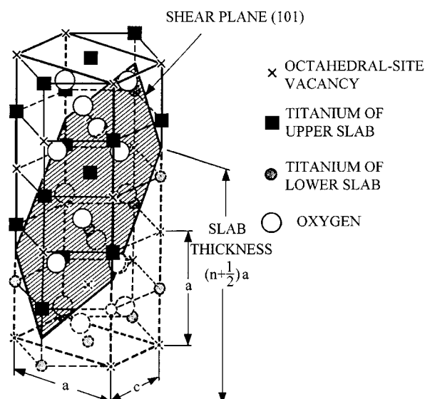
Fig. 2. Unit cell projection of the shear plane in the Magnéli phase Ti 4 O 7 . c , a and (1 0 1) refer to axes of rutile slabs [6].
