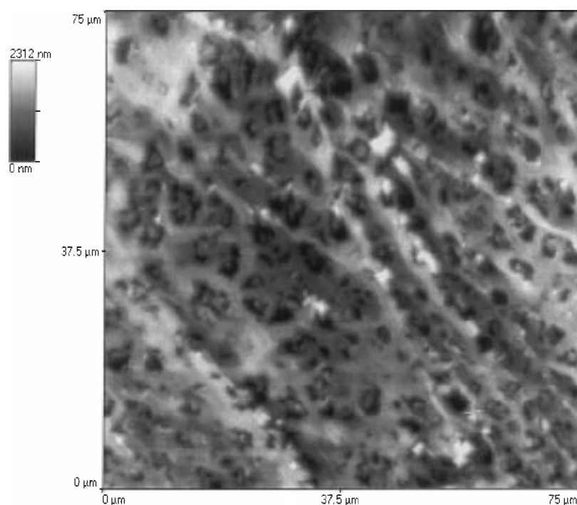
Fig. 6. Atomic force micrograph of a 'Flexible' Ebonex® electrode development, a composite material containing 85% by weight Ebonex® powder in a polyethylene matrix. Imaging parameters same as those stated for Fig. 5.
