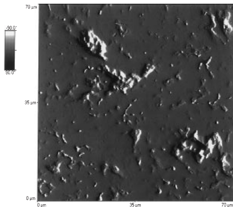
Fig. 5. An atomic force micrograph of a typical porous Ebonex® electrode. Image obtained in contact mode in air using a standard profile silicon nitride tip, 200 \mu\text{m} length 'V-shaped' cantilever of spring constant 0.038 \text{ N m}^{-1} and a force of 5 nN [39].
