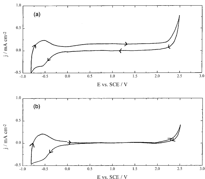
Fig. 7. Electrochemical behaviour of an Ebonex® material in 1 mol dm -3 sulphuric acid: (a) 1st scan commencing at 0 V and scanning to negative potentials, and (b) 2nd scan, 0 V to positive potentials. dE/dT = 50 \text{ mV s}^{-1} ; T = 298 \text{ K} [11].
